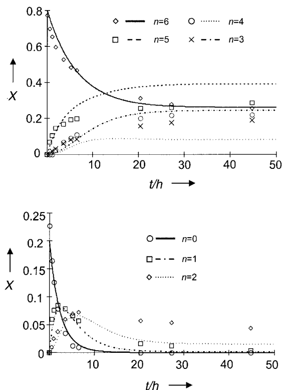
Figure 4. Time-dependent concentration of different species ( x = 1 mole fraction) [\text{Ga}_4\text{L}_n^2\text{L}_{6-n}^3 \supset (\text{Et}_4\text{N})]^{11-} as determined by NMR spectroscopy (points) and calculated according to a statistical model (lines) from a mixture containing pure [\text{Ga}_4\text{L}_6^2 \supset (\text{Et}_4\text{N})]^{11-} and [\text{Ga}_4\text{L}_6^3 \supset (\text{Et}_4\text{N})]^{11-} in a 4:1 ratio initially ( \text{D}_2\text{O} solution at \text{pD } 7.5 at 60^\circ\text{C} ).
